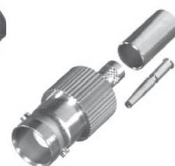
FIG. 54 RFB-1123-1, -1-SS, -C1, -C2, RFB-1124-1P, -1X
